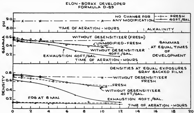
FIG. 4. Effect of aeration of an elon-borax developer containing a desensitizer (Formula D-89).
